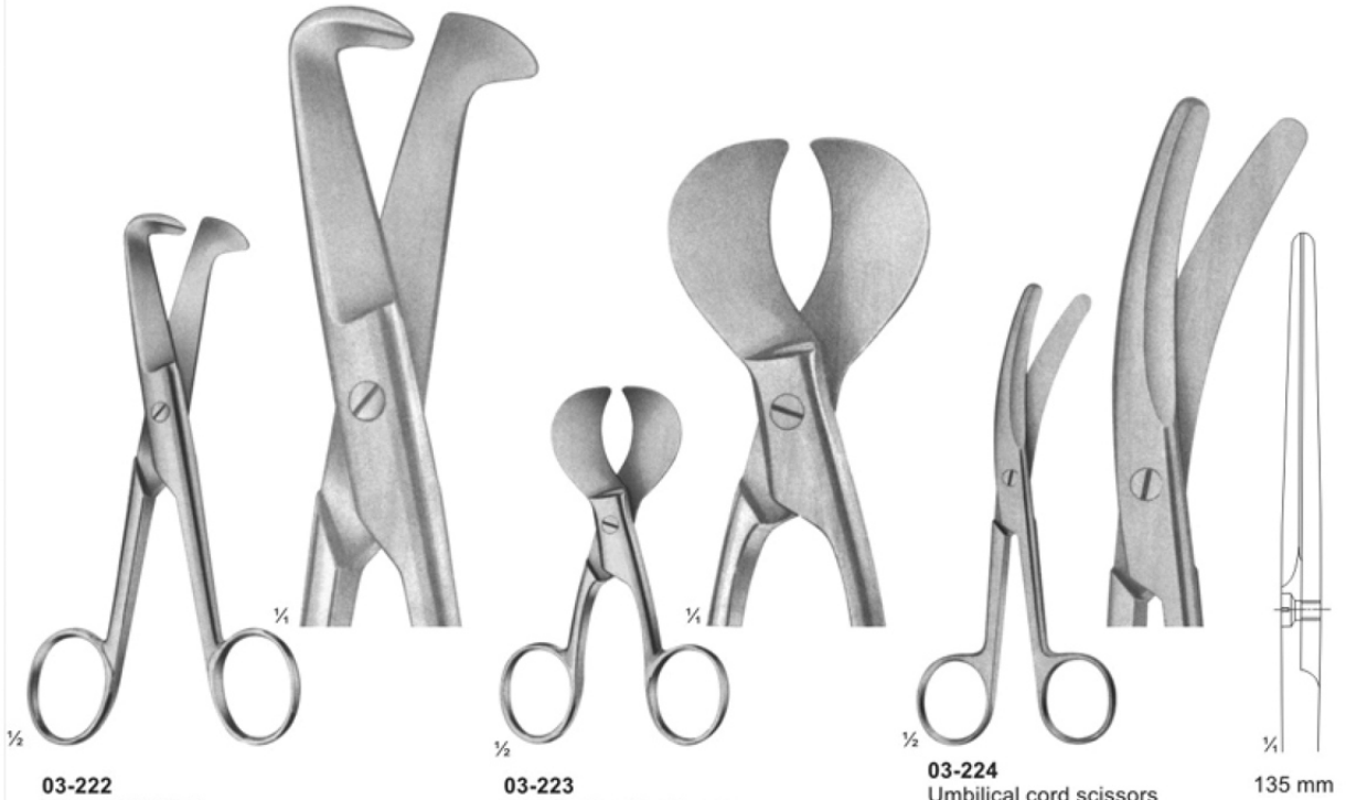
03-222 SCHUMACHER Umbilical cord scissors Size: 155 mm
